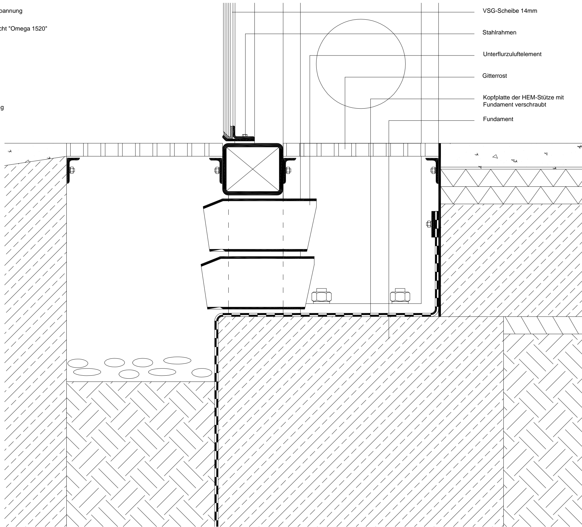
Pos.3 - Sockel
